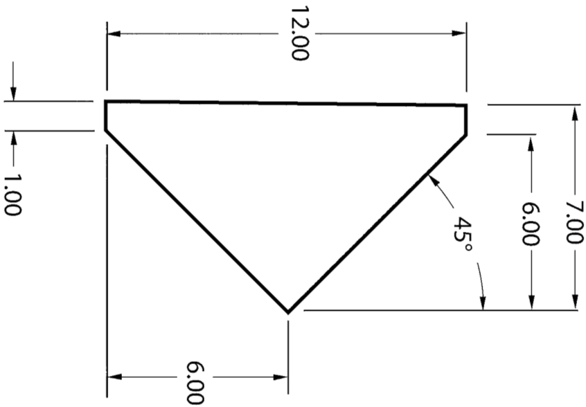
45° Fixture
